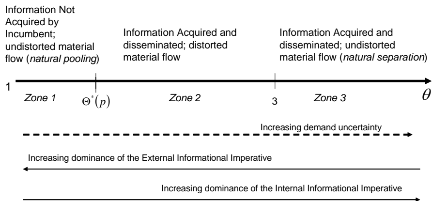
Figure 2: The equilibrium of the Information Acquisition Game.
