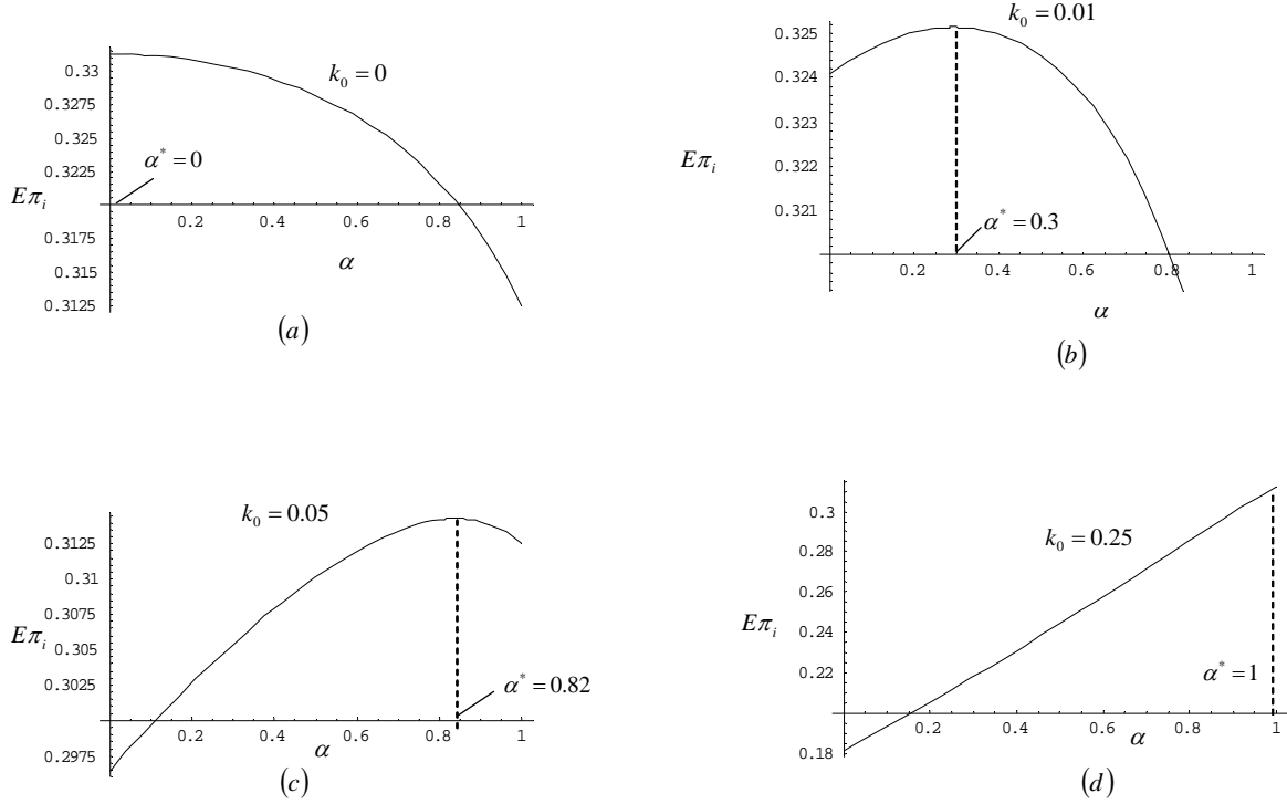
Fig. 3: Incumbent's expected profit ( E\pi_i ) as a function of \alpha and k_0 for p = 0.5, \theta = 2 . \alpha^* denotes optimal \alpha .
