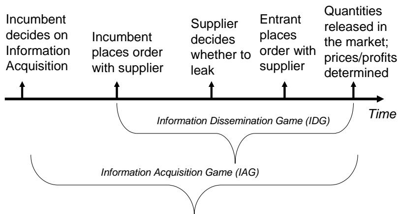
Figure 1: The Sequence of Events
