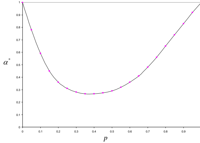
Figure 4: \alpha^* as a function of p for k_0 = 0.01, \theta = 2 .
